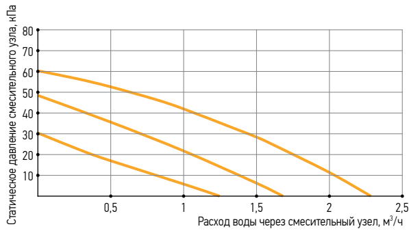
ONX 60-4,0
