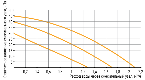
ONX 40-4,0
