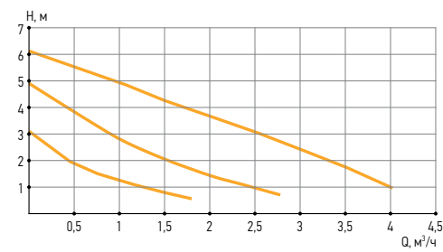
RS25-6G-180
