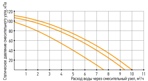
ONX 110-16,0
